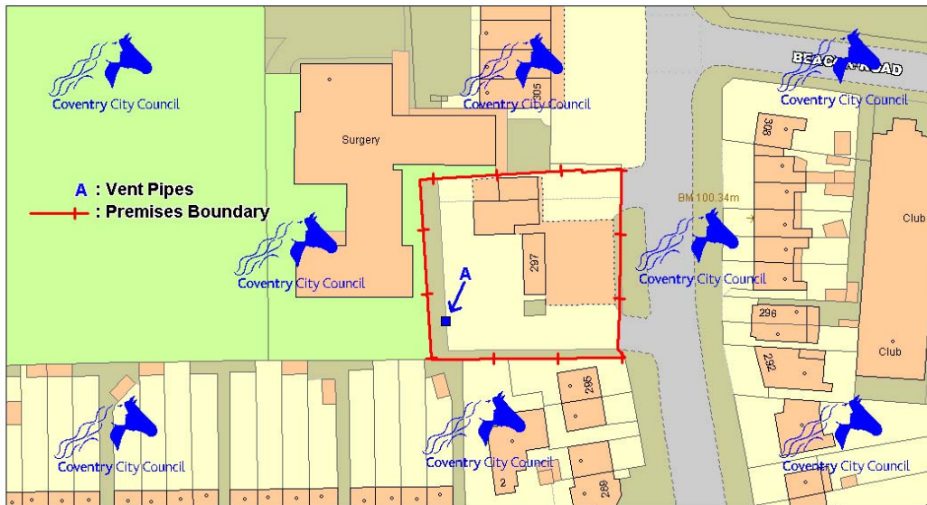
Plan PPC/124/A Shell Whitmore Park
