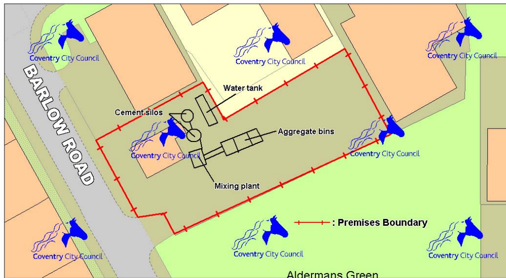
Plan PPC/023/A Premises Boundary of Tarmac Topmix
